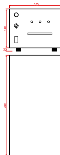
Power Supply Dimension:
